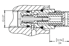
Anticavitation Valve
