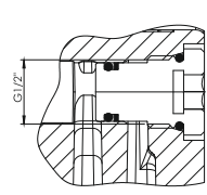
Cavity plug
